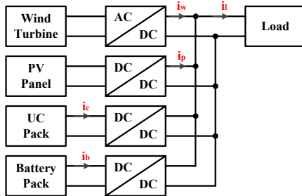
Fig. 2. System topology.
