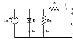
(a) Single PV cell.
