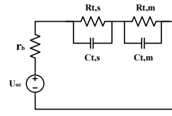
(b) Battery pack.
