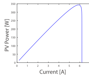
(a) PV power curve.
