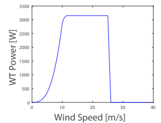
(b) WT power curve.
